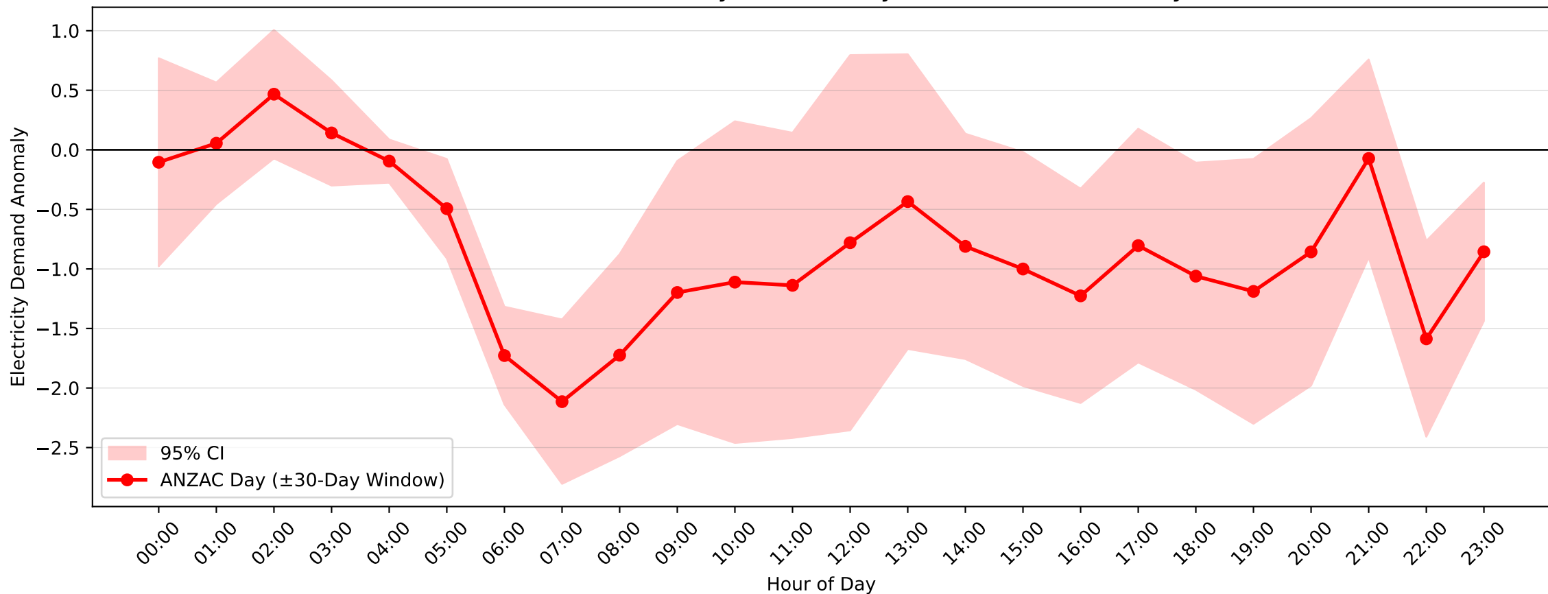
Charlestown Demand Anomaly: ANZAC Day (2004–2017, \pm 30 -Day Window)
